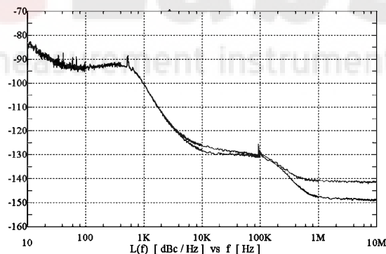
fc = 1.8 GHz (CW and I/Q modulation on)
