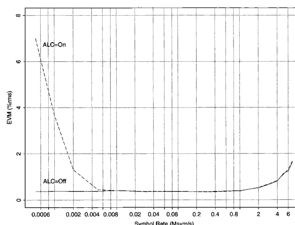
Effects of automatic level control (ALC) on EVM performance (fc = 1 GHz, root Nyquist filter, a = 0.25 , modulation = QPSK)
